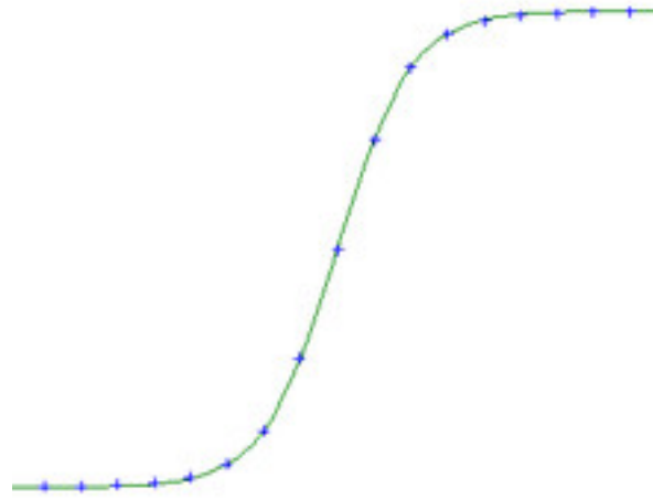
Figure 3: Sigmoid function.
